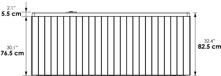
Vista lateral / Lateral view
