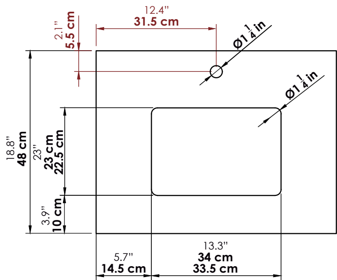
Vista top / Top view
