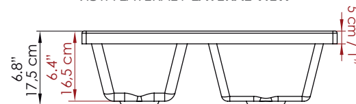
VISTA LATERAL / LATERAL VIEW
