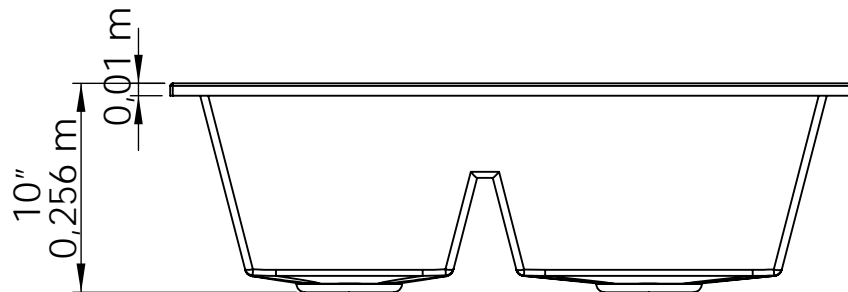
VISTA FRONTAL / FRONT VIEW
