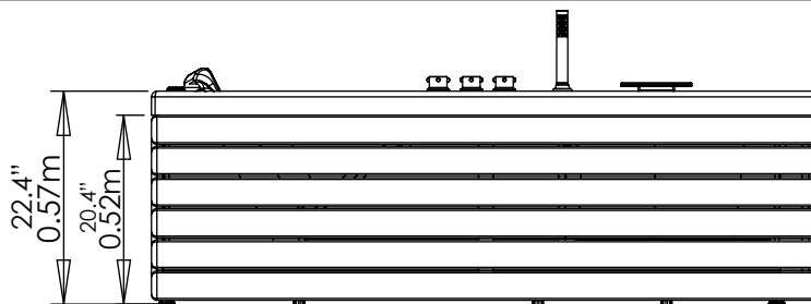
VISTA LATERAL / LATERAL VIEW
