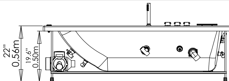
VISTA LATERAL / LATERAL VIEW
