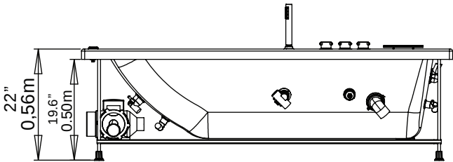
VISTA LATERAL / LATERAL VIEW
