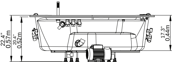
VISTA LATERAL / LATERAL VIEW
