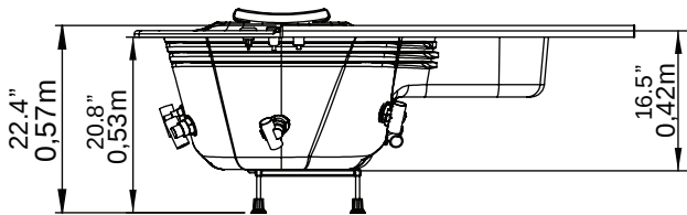
VISTA LATERAL / LATERAL VIEW
